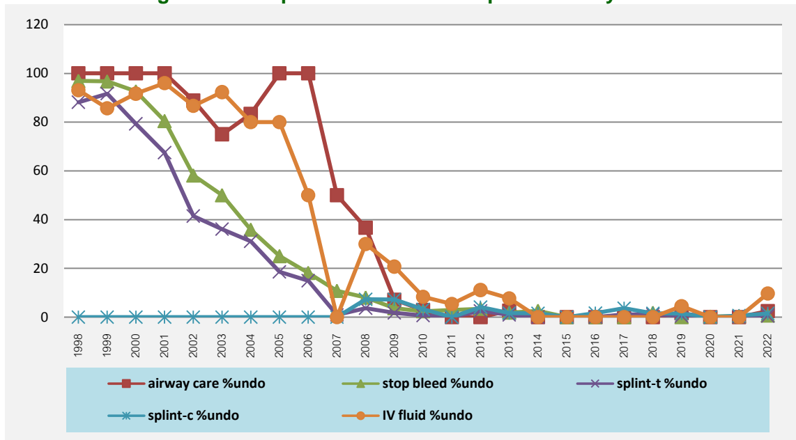
Figure 75 Comparison undo critical procedure by EMT
