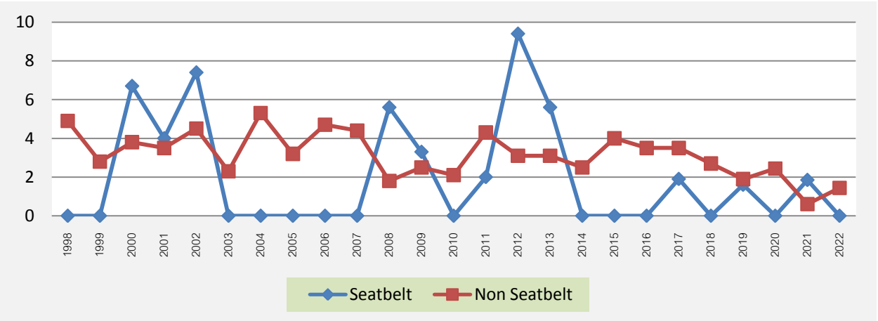
Figure 38 Passenger death rate of seatbelt and non-seatbelt used (1997-2022)
