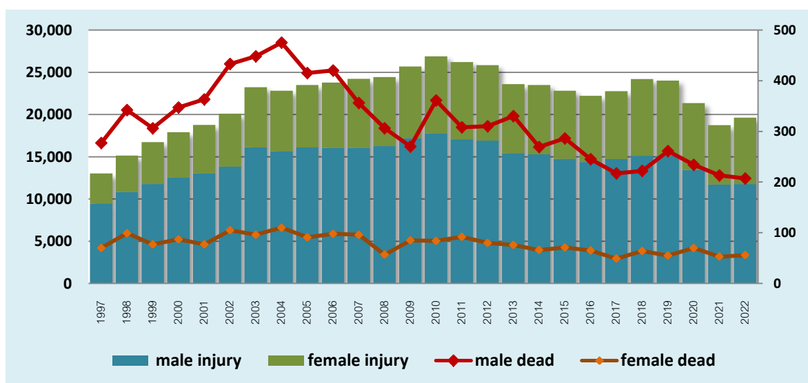
Figure 1 Number of injuries and deaths by gender (1997-2022)
