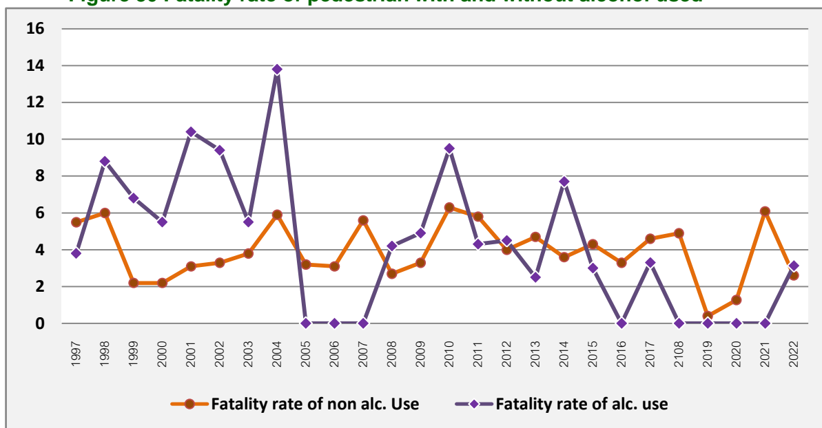
Figure 30 Fatality rate of pedestrian with and without alcohol used
