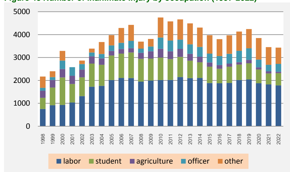
Figure 48 Number of inanimate injury by occupation (1997-2022)
