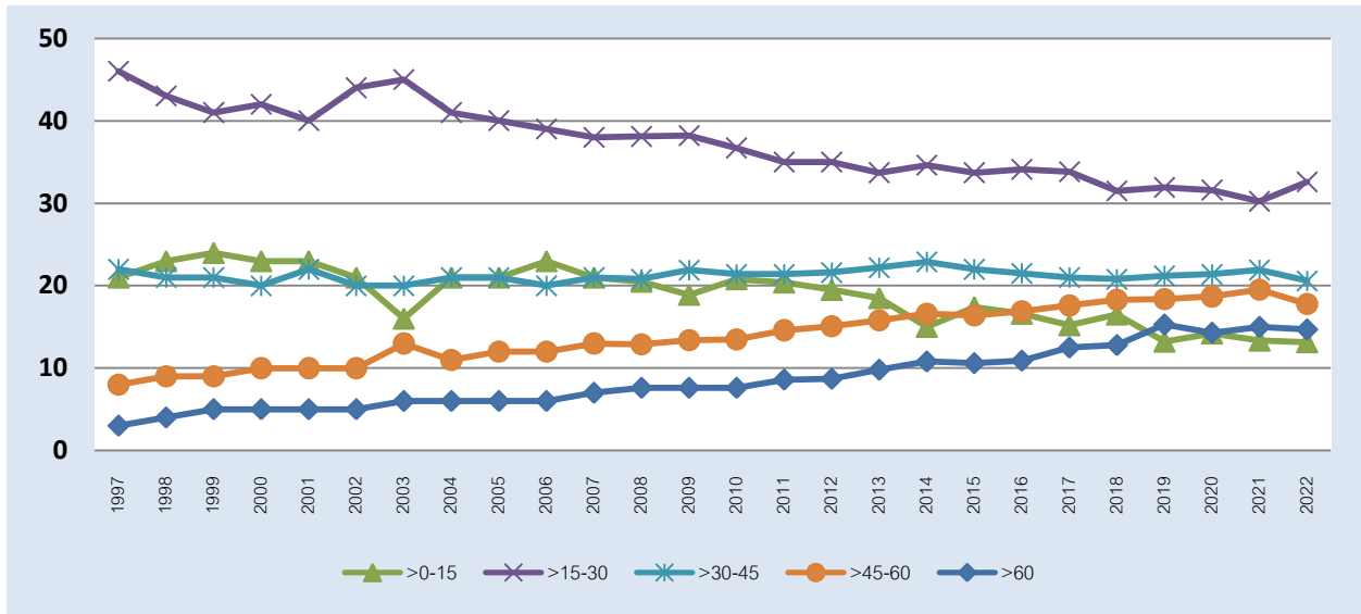
Figure 4 Percentage of injury by age group (1997-2022)
