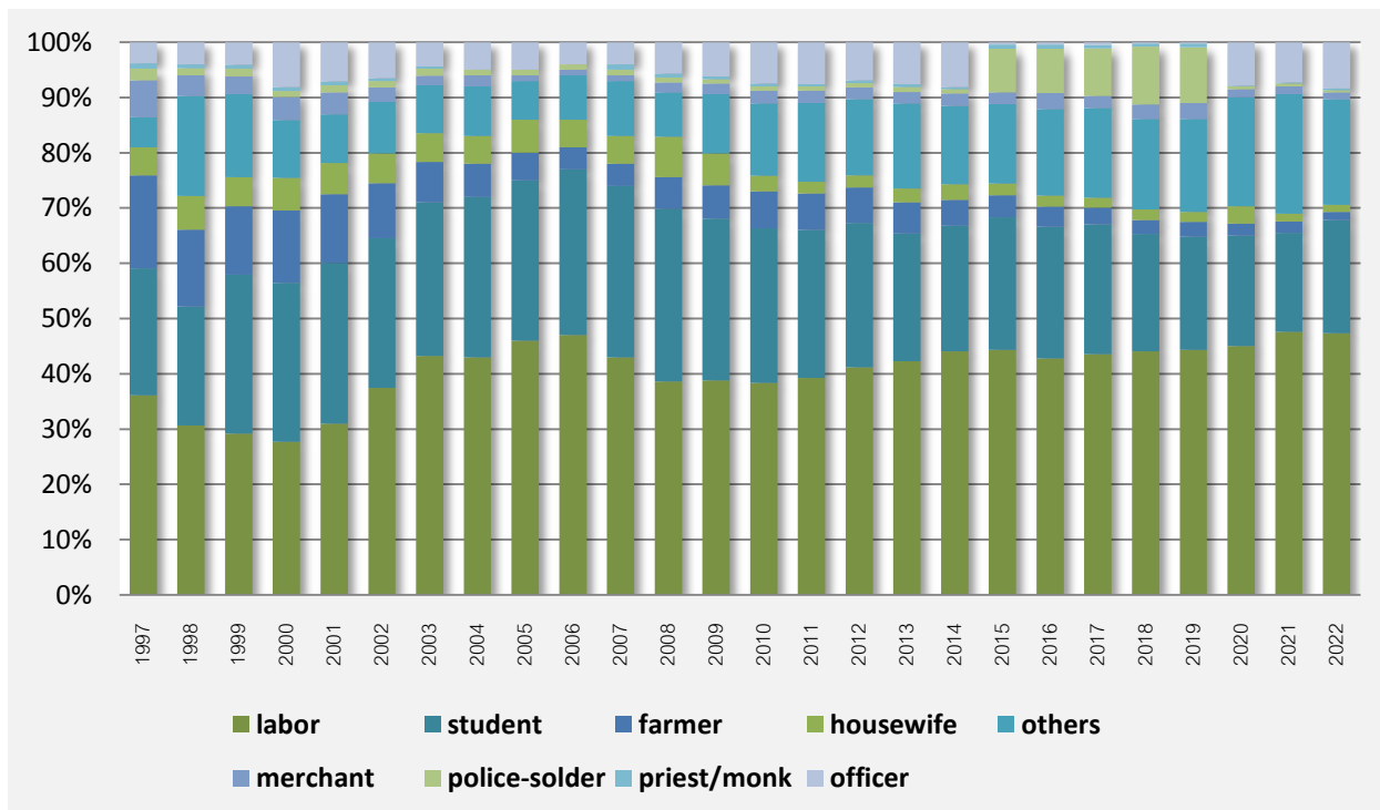
Figure 9 Percentage of injury by occupation (1997-2022)
