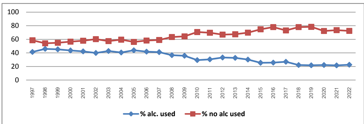
Figure 33 Proportion of motorcyclist death with & without alcohol used (1997-2022)
