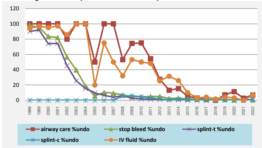
Figure 76 Comparison undo critical procedure in Volunteer
