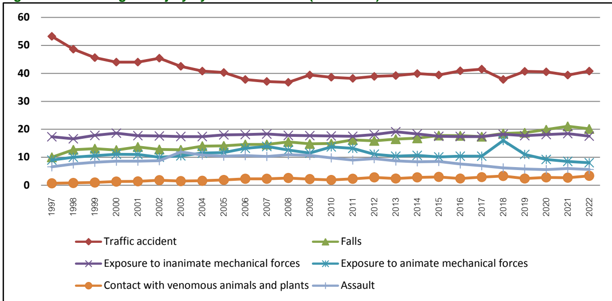
Figure 14 Percentage of injury by various causes (1997-2022)
