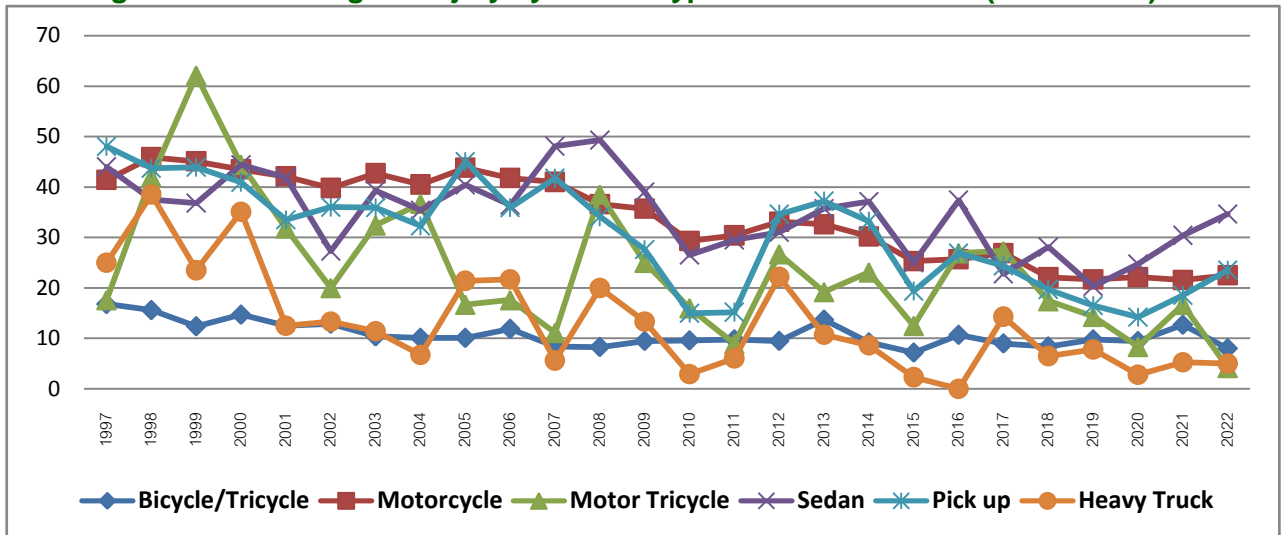
Figure 31 Percentage of injury by vehicle type with alcohol used (1997-2022)
