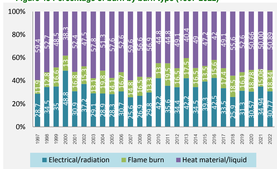
Figure 45 Percentage of burn by burn type (1997-2022)
