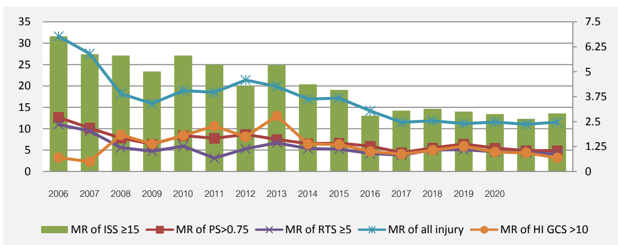
Figure 78 KPI for quality improvement in admission trauma care 2006 – 2022
